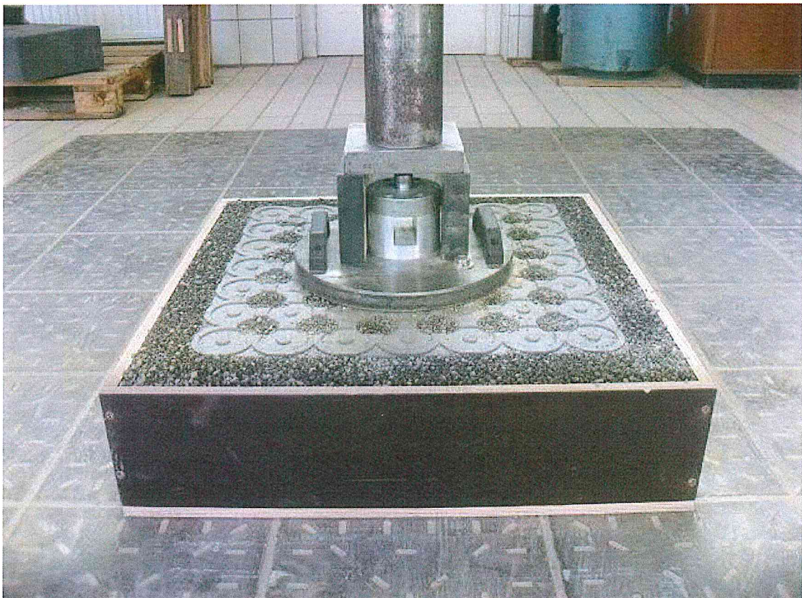
Figure 1: Test setup – "Cellular slabs Horses Home" on an artificially manufactured subgrade
